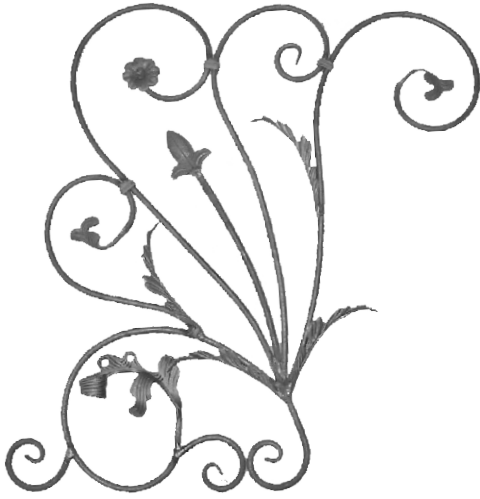
UP7063 12mm Round Bar Dim 760 x 890mm
